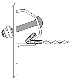
Bolt Type Clamp
