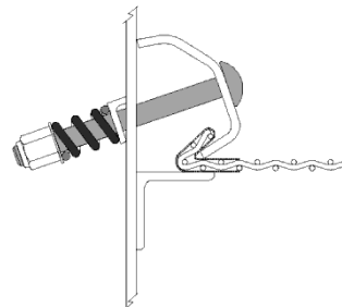
Spring type Clamp Bolt
